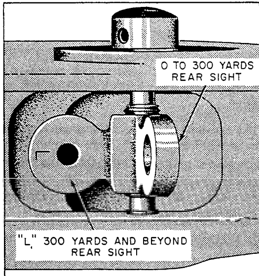
Figure 3-23.—Rear sight aperture.
