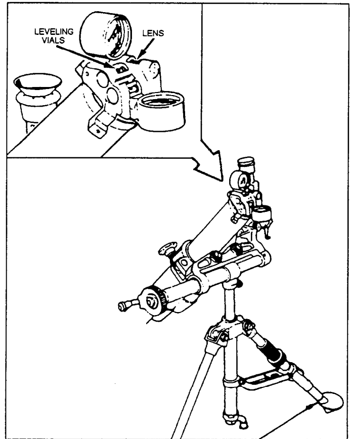
Figure 14-6.—Boresight (M115).
