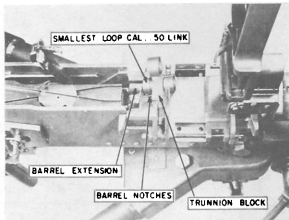
C-USING THE SMALLEST LOOP OF A .50-CAL LINK TO KEEP THE BARREL LOCKING SPRING LUG ALIGNED WITH THE 3/8-INCH HOLE.
