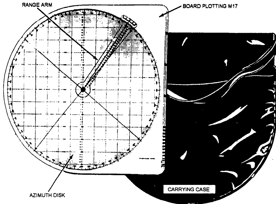
Figure 14-24.—Plotting board and carrying case.
